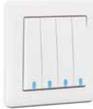
4G 2 Way Change-Over Switch Illuminated BR011601 20 A - 16 AX, 250 V~ BS EN 60669-1 Piece in Box / Package - 12 / 120
